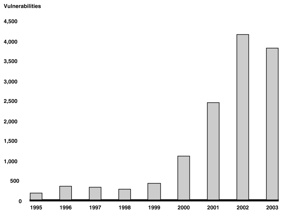
Figure 1: Security Vulnerabilities, 1995–2003
